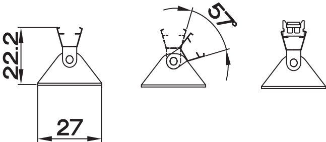
adjustable stainless fixing clip
