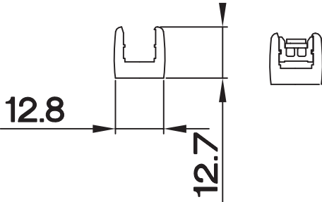
nylon fixing clip
