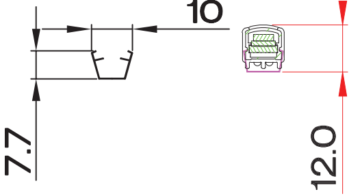
stainless steel fixing clip
