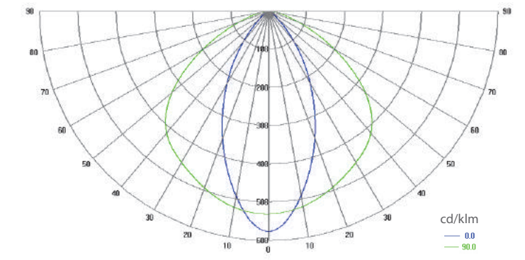
Polar Candela Distribution Plot Using Missed Rays
