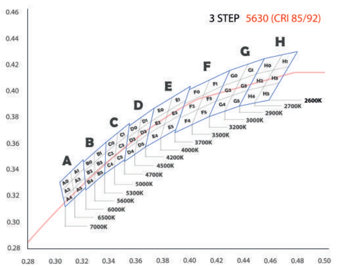
3 Step MacAdam Ellipse by default
