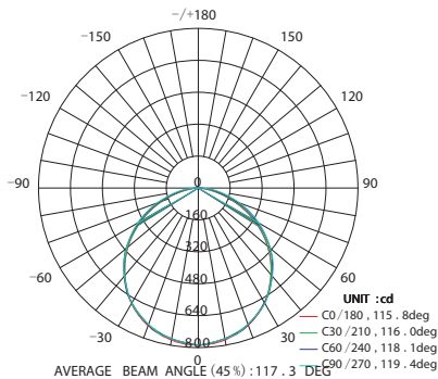
Light Distribution Curve(cd)
