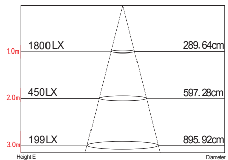
Lux distance curve(lux)
