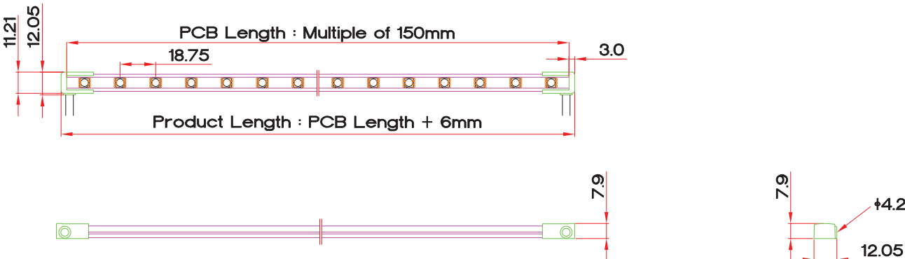
Straight end cap with fixing lug
